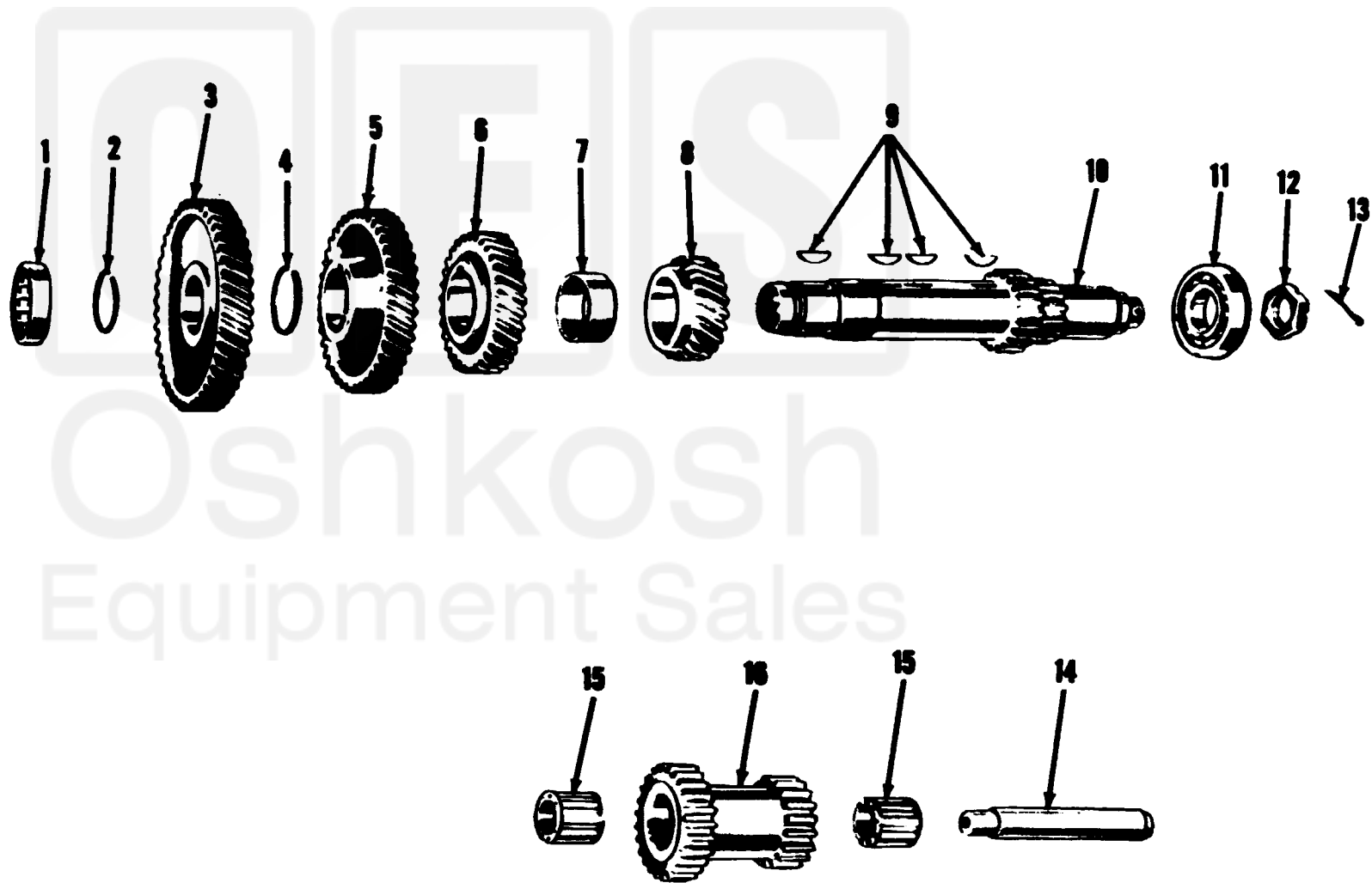
Figure 43. Transmission countershaft and idler shaft with gears—gasoline and multifuel.
